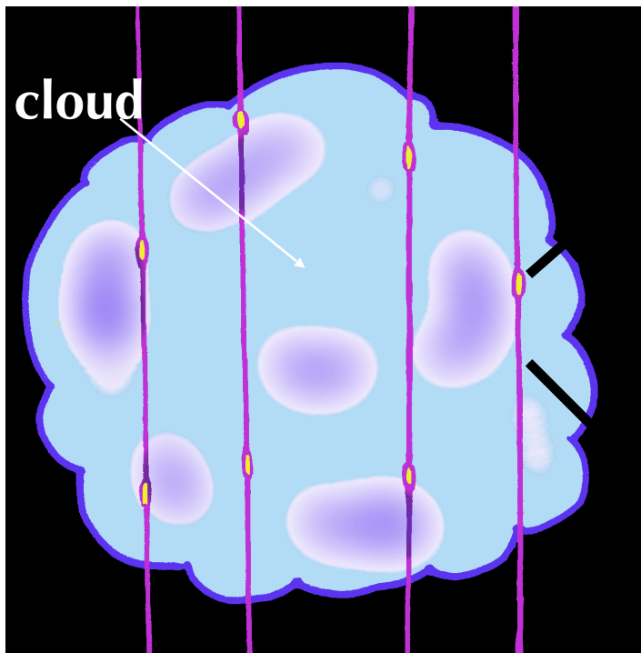
B lines across the ISM
