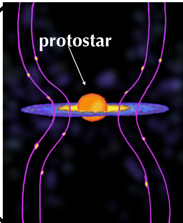
B lines drift during the collapse
